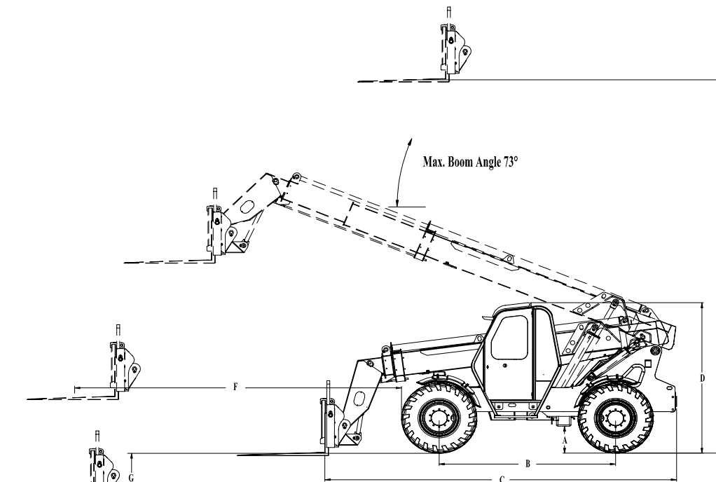
ARM 36' TELESCOPIC HANDLER
